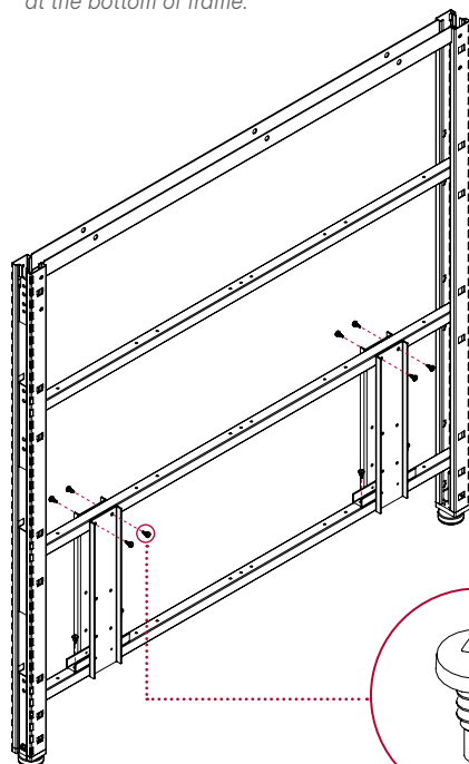
Vis autoperçante / Self-tapping screw #10 x 1/2" (6x)
